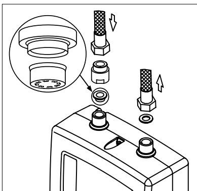
Installation with the outlet and inlet pipes on the top.
